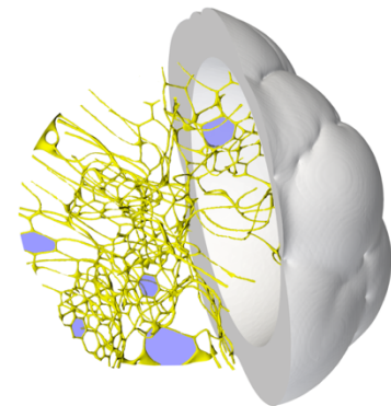
Figure: APFC simulation of the growth of a polycrystal npj Comput. Materials 5, 48 (2019)
